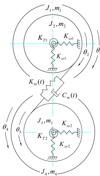
Fig. 3. Detailed gear pair model.
