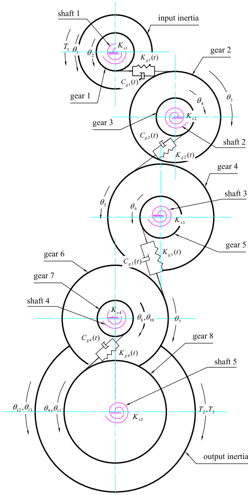
Fig. 2. Gear train model.
