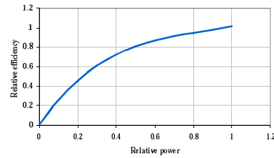
Figure 1. Relative engine efficiency (based on [39])
