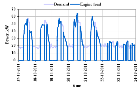
Figure 6. Demand vs optimal engine load
