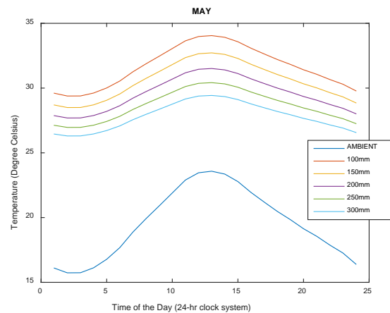
Fig.3.1: Generated internal brooder for various wall thickness. (Source: Authors, 2019)
