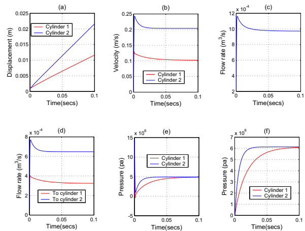
Fig. 21. Simulated open loop responses for case 3; (a) Piston displacements (b) Piston velocities (c) Pump flow rate (d) Flow rate to cylinders (e) Head sides chamber pressures (f) Rod side chamber pressures
