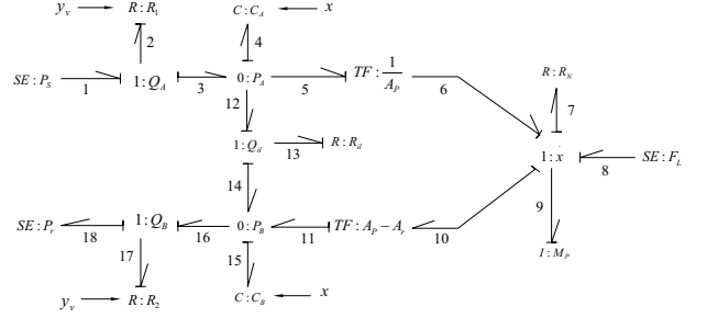
Fig. 14. A causal bond graph model for the cylinder during extension.
